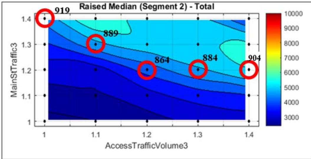
Figure D-3: Threshold volume analysis results for total conflicts
