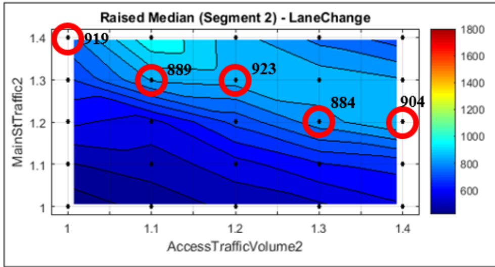
Figure D-2: Threshold volume analysis results for lane-change conflicts
